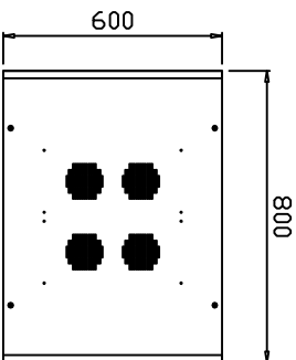
PLAN VIEW
