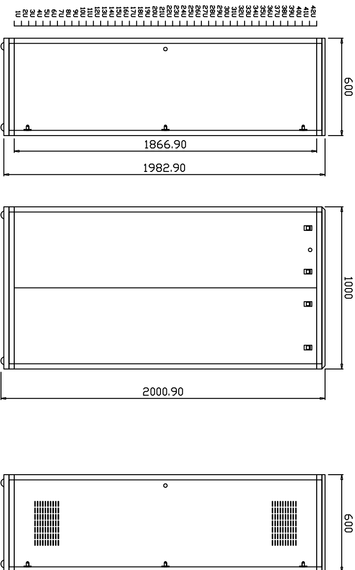
PLAN VIEW
