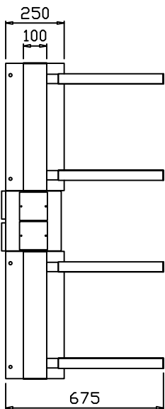
PLAN VIEW
