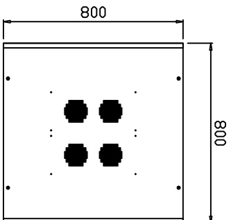
PLAN VIEW
