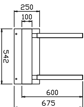
PLAN VIEW
